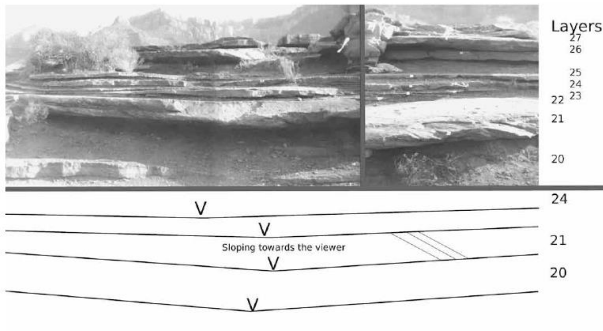
Figure 6. Composite view of Tapeats layers described here. Camera angle in the far right photo was shifted to show above layers more distinctly. Numbering of layers and location of thalweg (V) in each layer is indicated. Lee slope depositional direction is visible in several locations in photo and indicated in diagram.
