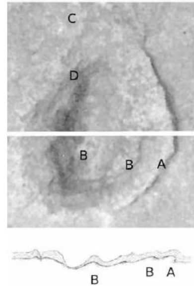
Figure 11. Impression 2 with cross section, showing (A) original push-up produced by shear action, (B) secondary push-up, (C) push-up relocated by moving water, and (D) the multiple layers affected.
